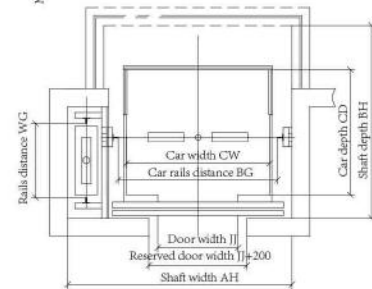
Shaft layout(square)
